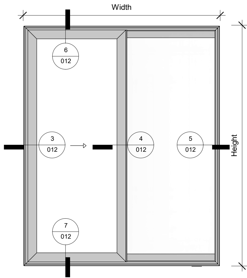
1 Elevation Front 1 : 20
